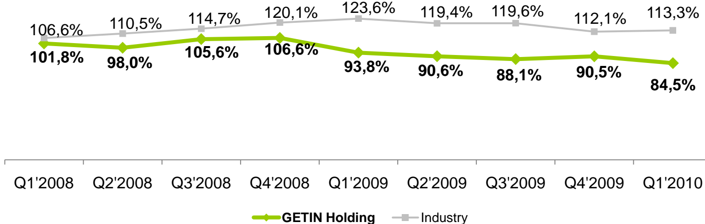
Credits/Deposits ratio(%)
